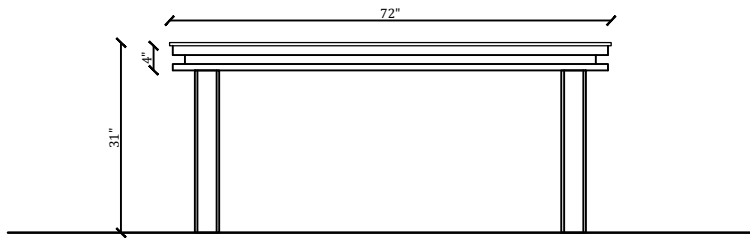
DINING TABLE FRONT VIEW
