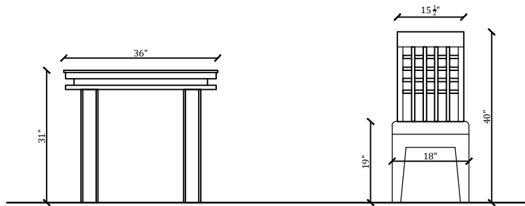
SIDE VIEW OF DINING TABLE
